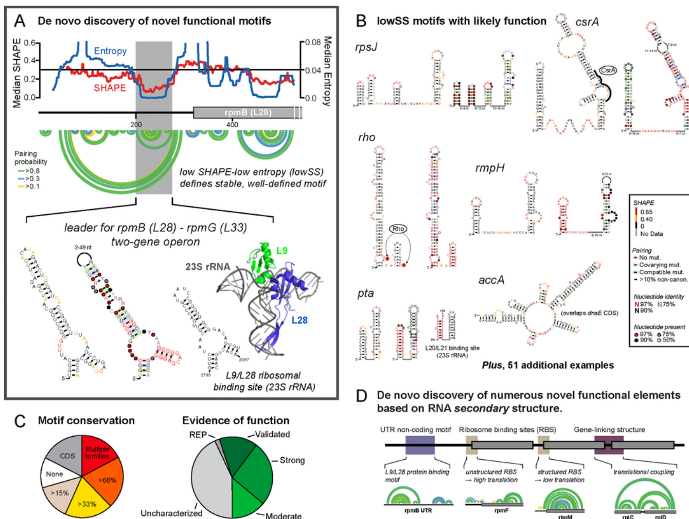
Figure 8. De novo discovery of functional RNA elements as lowSS regions. (A) LowSS region (gray box) in the rpmB mRNA forms an autoregulatory element that mimics L9/L28 binding sites in the 23S rRNA. (B) Novel RNA regulatory elements identified in E. coli . Structures are annotated by SHAPE reactivity and evidence for conservation. (C) Conservation of lowSS structures identified in enterobacteria and evidence of function based on literature. (D) Mechanisms by which RNA structure regulates gene expression across the E. coli transcriptome based on identification of well-determined secondary structures. 2 Arcs indicate base pairs.
