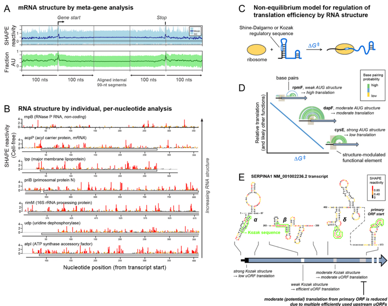
Figure 7. Structural personalities of bacterial and human RNAs. (A) Metagene representation of averaged mRNA structure in E. coli based on SHAPE reactivity and A/U nucleotide content. (B) Per-nucleotide SHAPE reactivities for one lncRNA and six mRNAs from E. coli . 2 (C) Model for how RNA structure modulates accessibility to regulatory sequences. Unfolding an RNA motif ( \Delta G^\ddagger ) imposes an energetic penalty on translation initiation (and likely many other processes). (D) RNA structures that tune translation initiation in E. coli . Brown box indicates AUG translation start site; arcs illustrate RNA base pairs. (E) Example of SERPINA1 mRNA structure containing a primary ORF and three ( \alpha , \beta , \delta ) competing upstream open reading frames (uORFs). Minimum free energy structures are shown, nucleotides are colored by SHAPE reactivity, and Kozak sequences are boxed.
