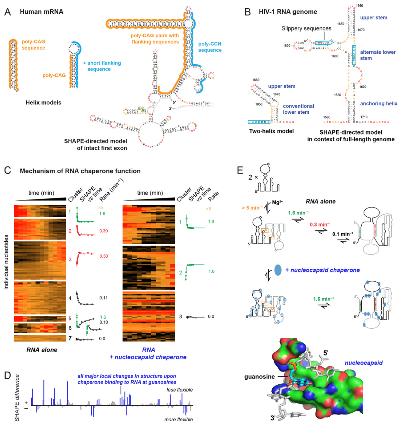
Figure 5. Comprehensiveness in understanding RNA structure and RNA–protein interactions. (A) Secondary structure models for CAG repeat-containing sequences from human HTT mRNA based on analysis of (left) local structures and (right) the full-length first exon (360–500 nt, depending on number of CAG repeats). Adapted from ref 77. Copyright 2013 American Chemical Society. Start codon is boxed in green. (B) Secondary structure models of the HIV-1 RNA frameshift element based on analysis of (left) local structure and (right) the entire HIV-1 genome. Reproduced from ref 78. Copyright 2014 American Chemical Society. (C) Time-resolved folding of a retroviral RNA packaging domain in the absence and presence of nucleocapsid chaperone. 83 Per-nucleotide reactivities are shown on a scale from red (high) to black (low). Nucleotides are grouped by k -means clustering; kinetic profiles are shown for each cluster. (D) SHAPE-detected protein–RNA contacts 7 s after protein addition reveal interactions at guanosine (blue). (E) Model for chaperone-mediated facilitation of RNA folding by destabilizing interactions involving guanosine. 83
