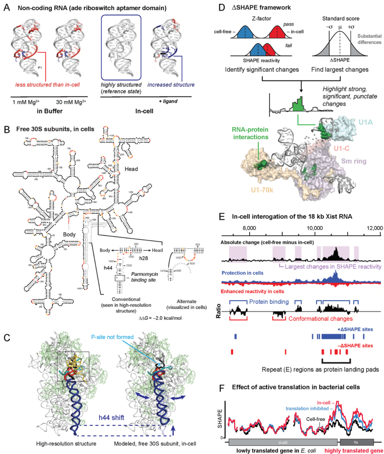
Figure 6. Cellular environment and RNA structure. (A) SHAPE analysis of the adenine riboswitch aptamer domain under simplified conditions, in cells (the reference state, box) and in the presence of ligand. 50 Higher and lower SHAPE reactivities relative to in-cell RNA are red and blue, respectively. (B) Model for the structure of the 16S rRNA in free 30S subunits in cells. 49 SHAPE reactivity pattern in helices 28 and 44 is incompatible with the structure visualized in high-resolution structures. (C) Movement of helix 44 in the in-cell state, emphasizing a large-scale conformational switch. (D) \Delta SHAPE framework for identifying significant changes between two states. Structure shows \Delta SHAPE sites in the human U1 snRNP complex (green spheres) and their proximal proteins. (E) Protein interactions across the mouse Xist lncRNA mapped using large-scale difference analysis. (top) Effects of the in-cell environment categorized by absolute differences in SHAPE reactivity (50 nt sliding window). (middle) Ratio of positive to negative differences is suggestive of protein binding and RNA structural rearrangement. (bottom) Positive and negative \Delta SHAPE sites are blue and red, respectively. (F) Effect of translation on RNA structure in E. coli cells. SHAPE reactivities increase, relative to the cell-free state, specifically in highly translated genes; kasugamycin treatment partially abrogates this increase.
