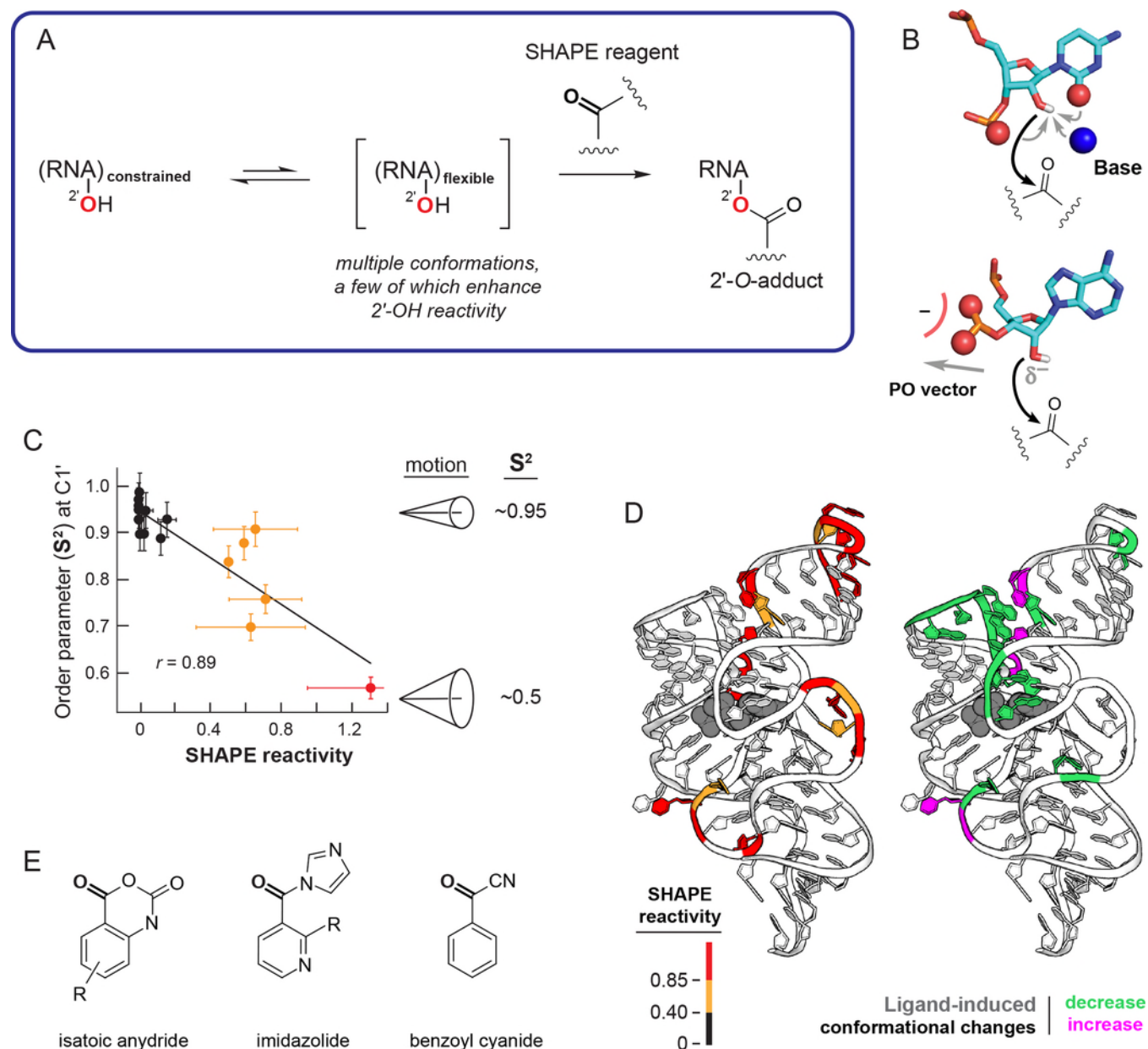
Figure 2. Mechanism of RNA SHAPE chemistry. (A) Reaction scheme. (B) Nucleotide conformations that enhance SHAPE reactivity involve (top) general base catalysis by the pyrimidine O2 (or purine N3), pro-S oxygen, or through-space groups and (bottom) stabilization of the 2'-oxyanion via conformations that direct nonbridging oxygen groups away from the 2'-OH group. (C) Correlation between the model-free generalized order parameter, S^2 , and SHAPE reactivity, exemplified by the U1A-binding RNA element. Adapted from ref 33. Copyright 2008 American Chemical Society. (D) SHAPE reactivities superimposed on the TPP riboswitch aptamer domain showing (left) absolute SHAPE reactivities and (right) changes in SHAPE reactivities (and thus local nucleotide dynamics) upon ligand binding (gray). (E) Classes of SHAPE reagents.
